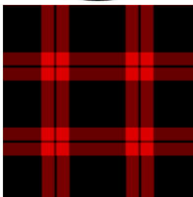
Red-Black check
